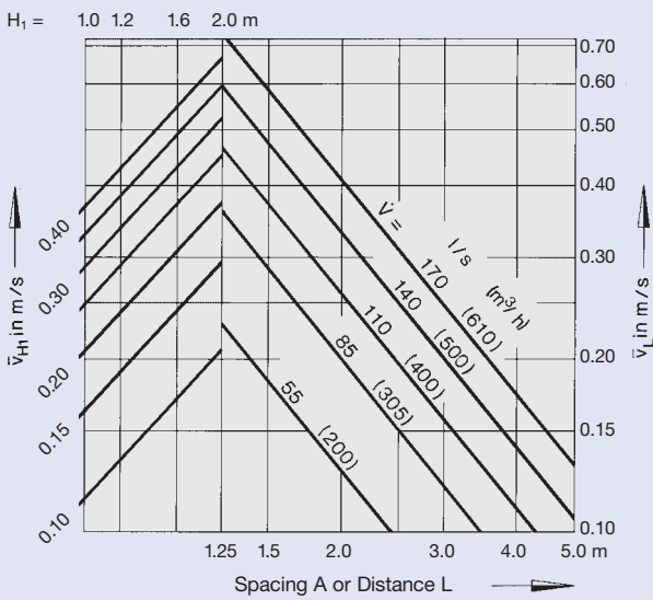
14 Air velocity Size 4
