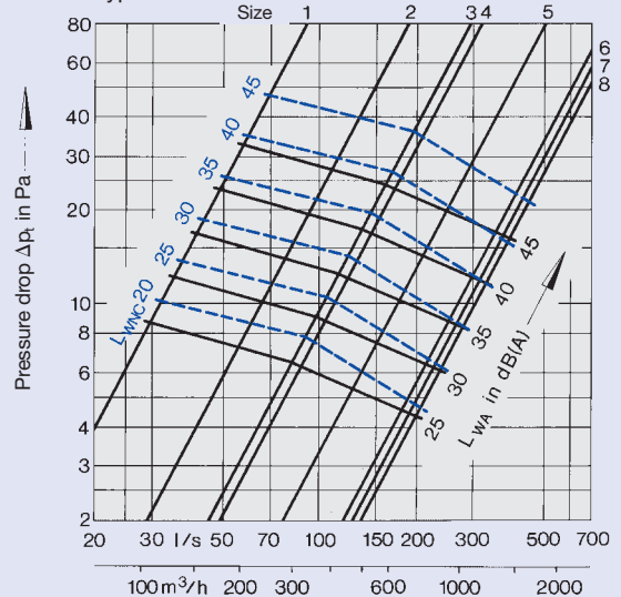
6 Sound power level and pressure drop Type ADLR-AV · ADLR-Q-AV
