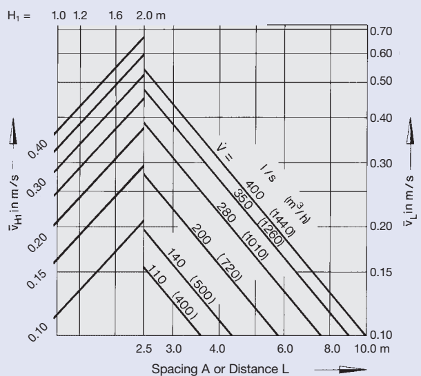
15 Air velocity Size 5
