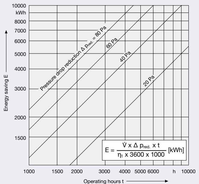
Energy saving by reduced pressure drop
