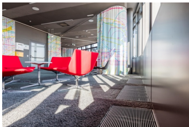
For the offices, under floor induction units BID from TROX were chosen, these being used for ventilation, heating and cooling.
