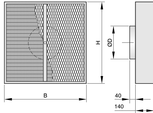
FHD – Construction with centre mullion
