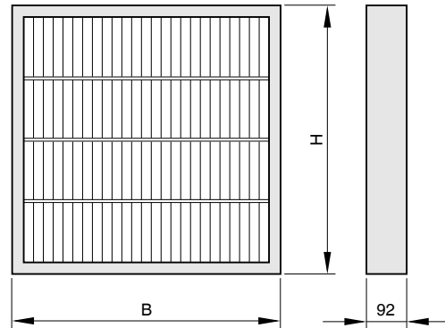
Dimensional drawing of ZL, 92 mm
