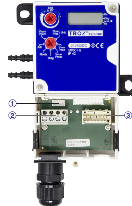
Universal controller XD4, type GUAC-SM3 (terminal cover opened)
