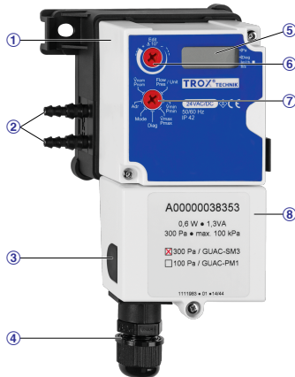
Universal controller XD4, type GUAC-SM3
